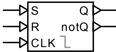
S-R flip-flop nor-gated
