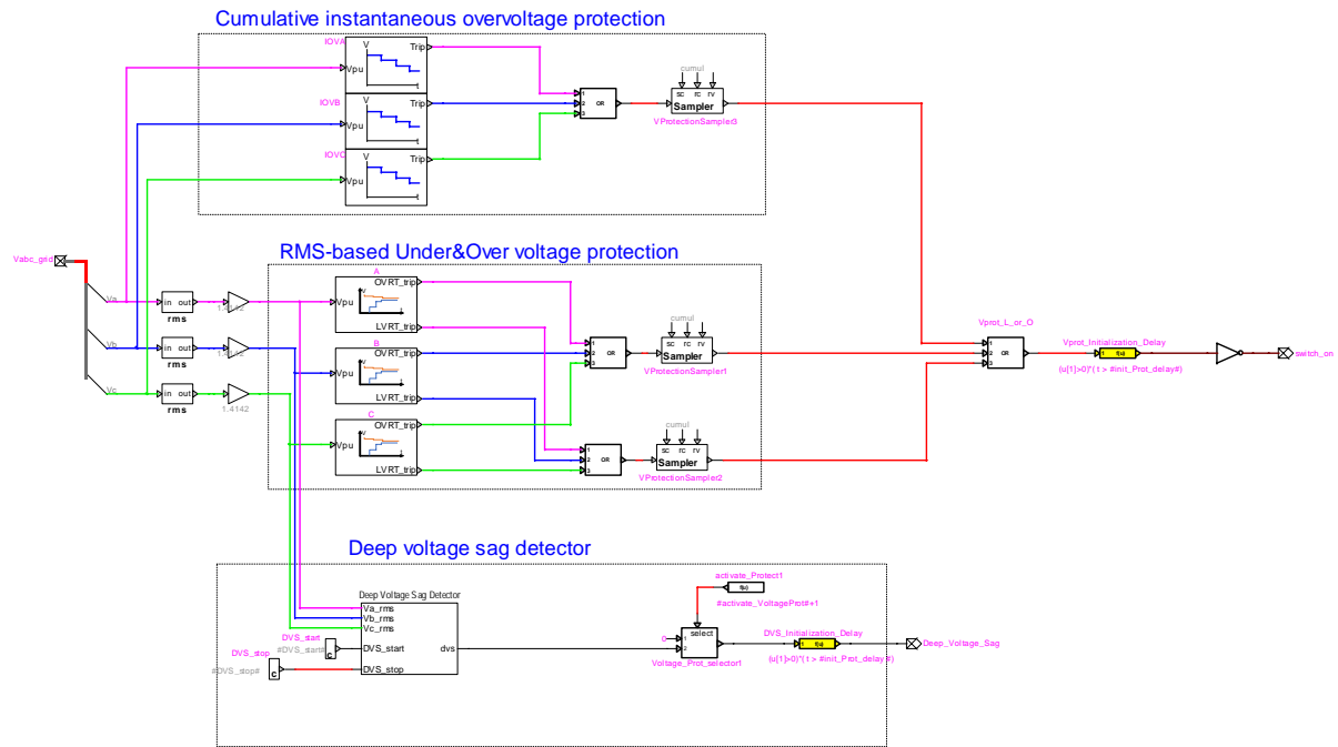
Figure 30 EMTP® diagram of overvoltage and undervoltage protections
