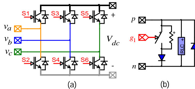
Figure 12 (a) Two-level Converter, (b) IGBT valve
