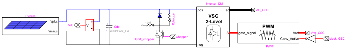
Figure 11 EMTP® diagram of dc-ac converter system block in PV models (detailed model version)
