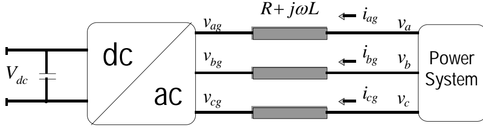
Figure 23 GSC arrangement
