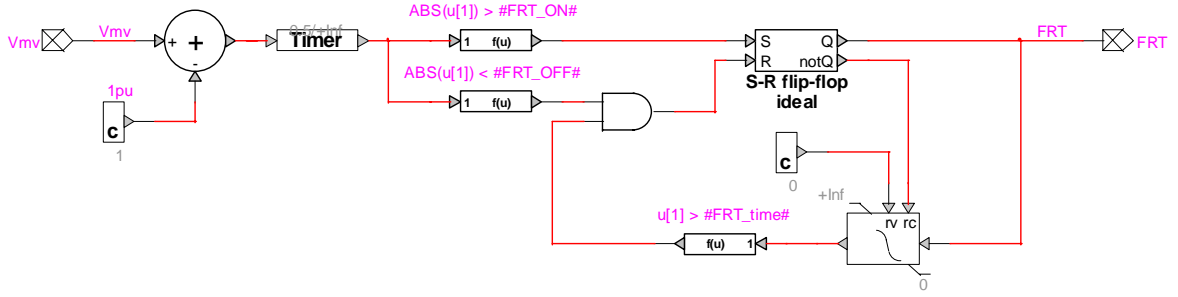
Figure 26 EMTP® diagram of “FRT decision logic” block
