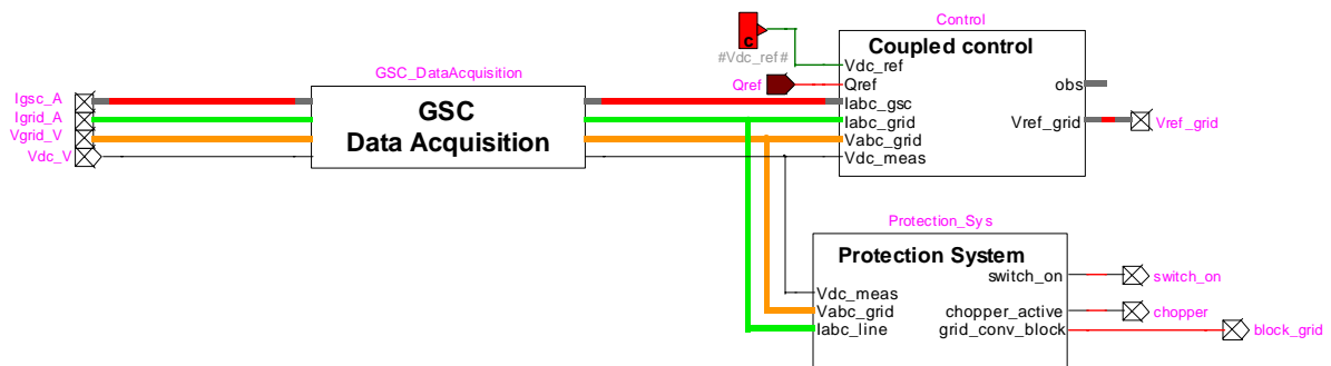
Figure 20 EMTP® diagram of the PV inverter control block
