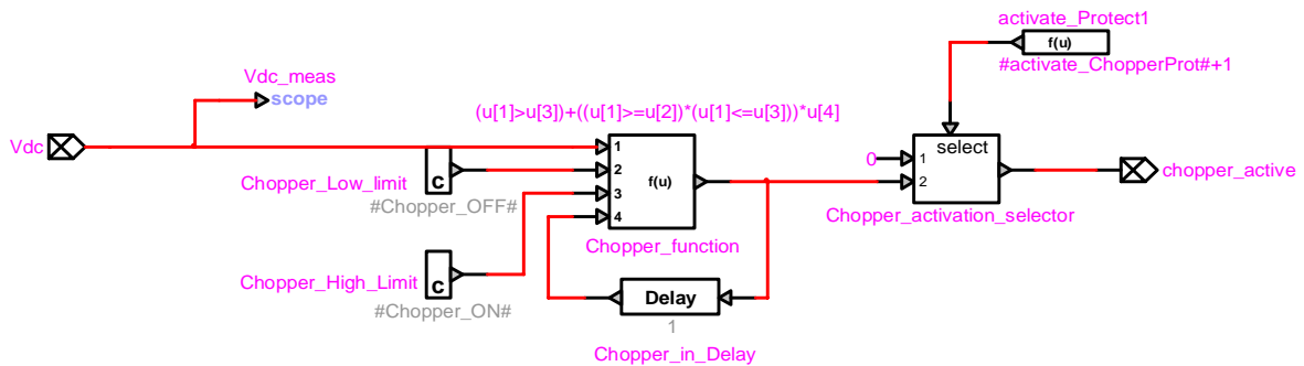
Figure 33 EMTP® diagram of dc overvoltage protection block
